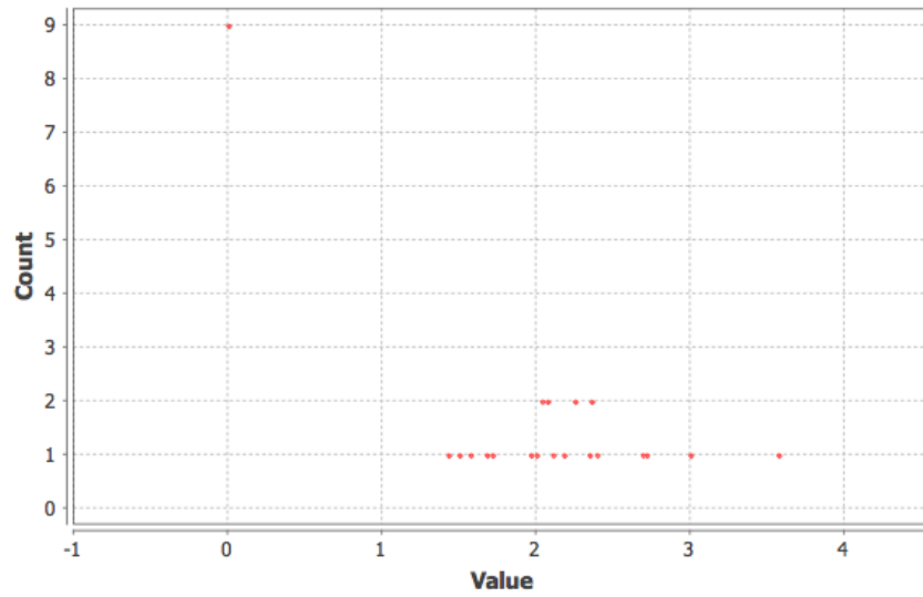
Eccentricity Distribution
