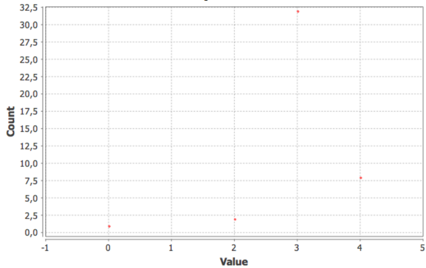
Eccentricity Distribution
