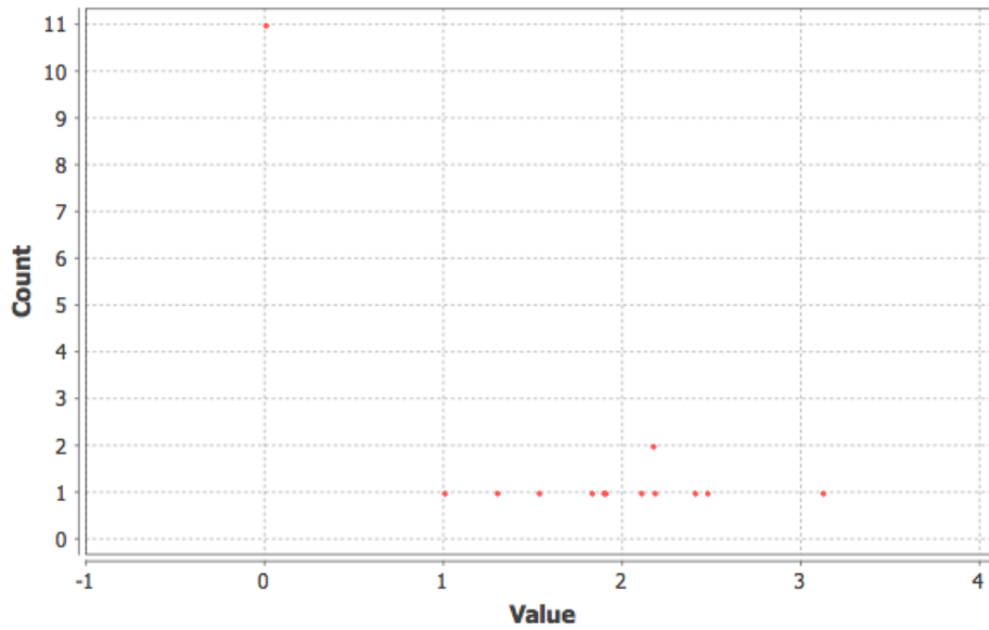
Eccentricity Distribution
