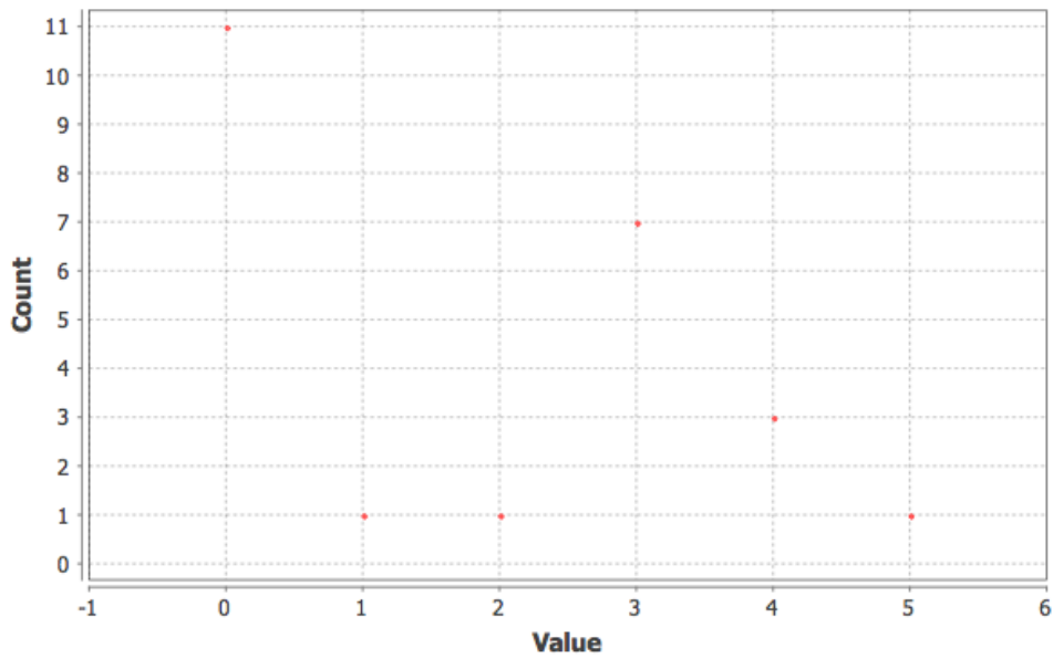
Eccentricity Distribution
