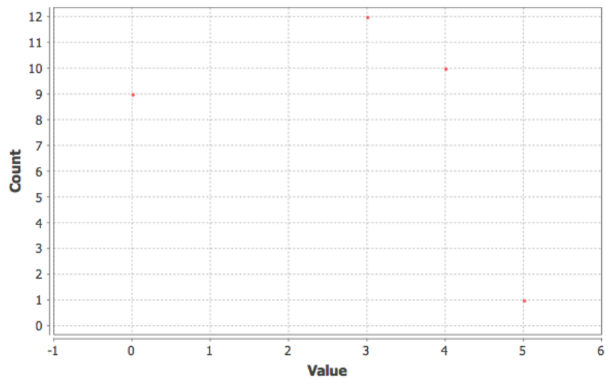
Eccentricity Distribution
