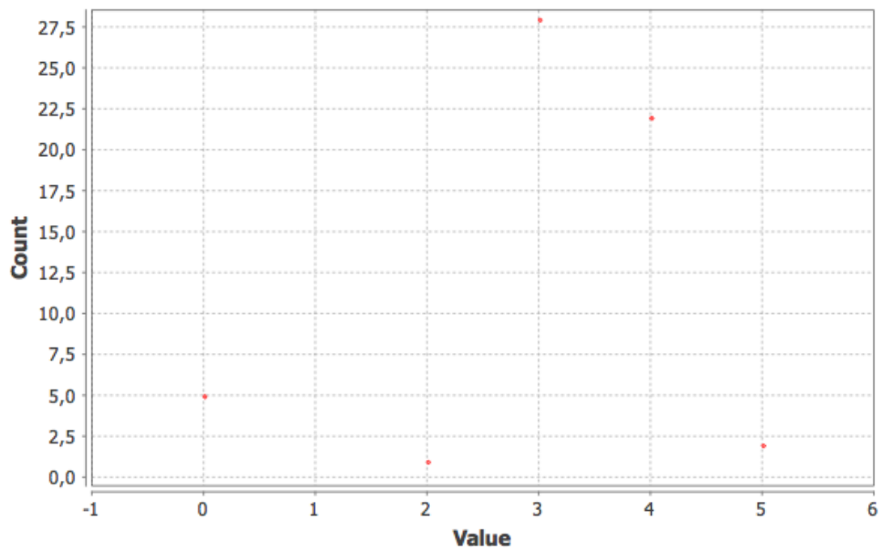
Eccentricity Distribution
